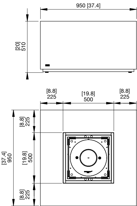
Line drawings show concrete models without a Fire Screen. Refer to the Fire Screen model specifications for dimensions.
